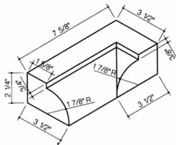
501-Watertable Inside Return Left
