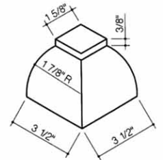
504-Watertable Outside Corner
