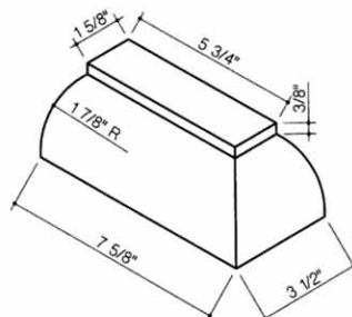
506-Watertable Outside Return Left
