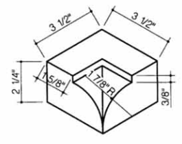
508-Watertable Inside Corner
