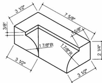
502-Watertable Inside Return Right
