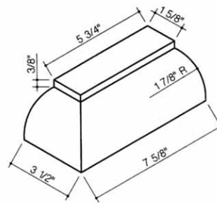
507-Watertable Outside Return Right
