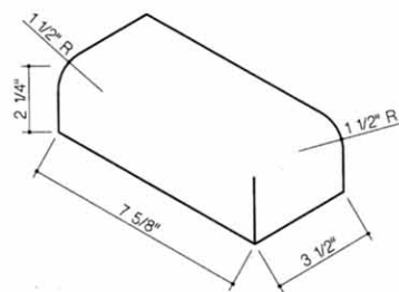
106- Bullnose Outside Return Left
