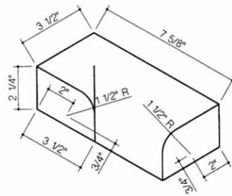
102- Bullnose Inside Return Right
