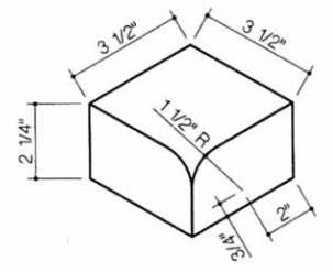
108-Bullnose Inside Corner
