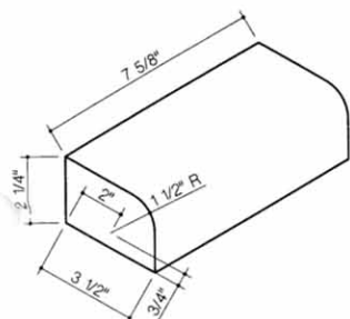
105- Bullnose Stretcher
