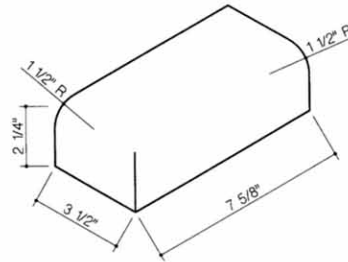
107-Bullnose Outside Return Right
