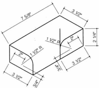
101-Bullnose Inside Return Left
