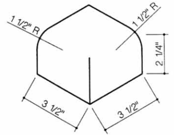
104-Bullnose Outside Corner
