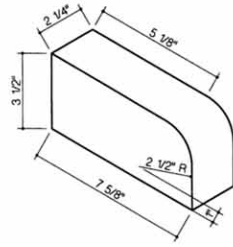
110-Rowlock Bullnose
