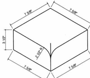
111-Rowlock Bullnose Inside Corner
