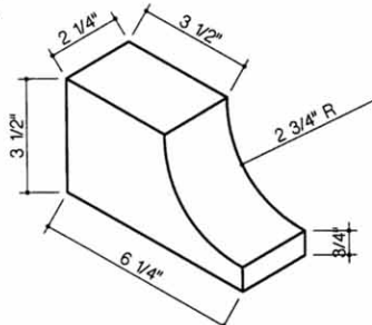
210-Rowlock Cove
