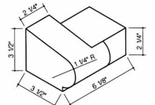
412-Window Sill Corner Right
