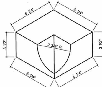
211-Rowlock Cove Inside Corner
