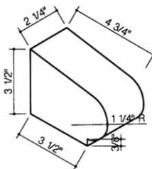
410-Window Sill
