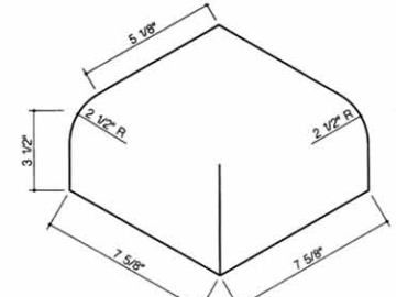
112-Rowlock Bullnose Outside Corner
