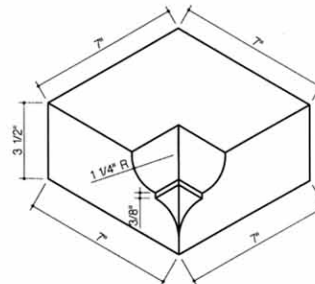
311-Ogee Rowlock Watertable Inside Corner
