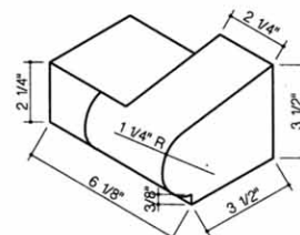
411-Window Sill Corner Left
