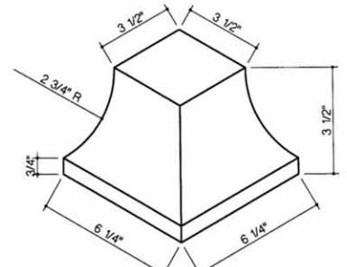
212-Rowlock Cove Outside Corner
