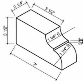
310-Ogee Rowlock Watertable
