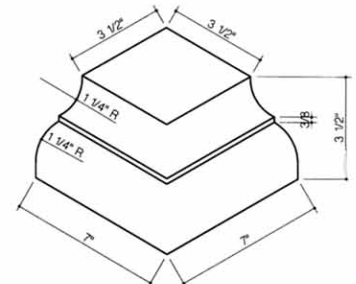
312-Ogee Rowlock Watertable Outside Corner
