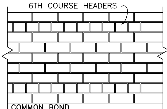
COMMON BOND
