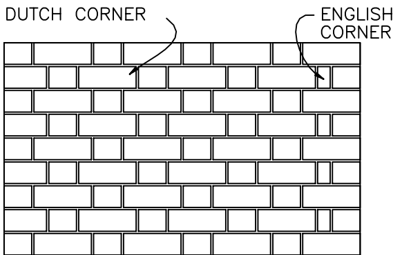
FLEMISH BOND
