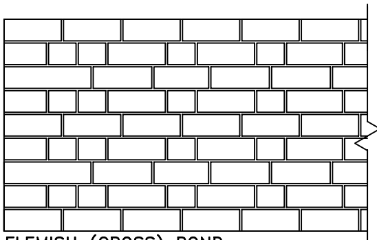
FLEMISH (CROSS) BOND
