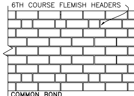
COMMON BOND
