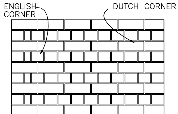
ENGLISH BOND
