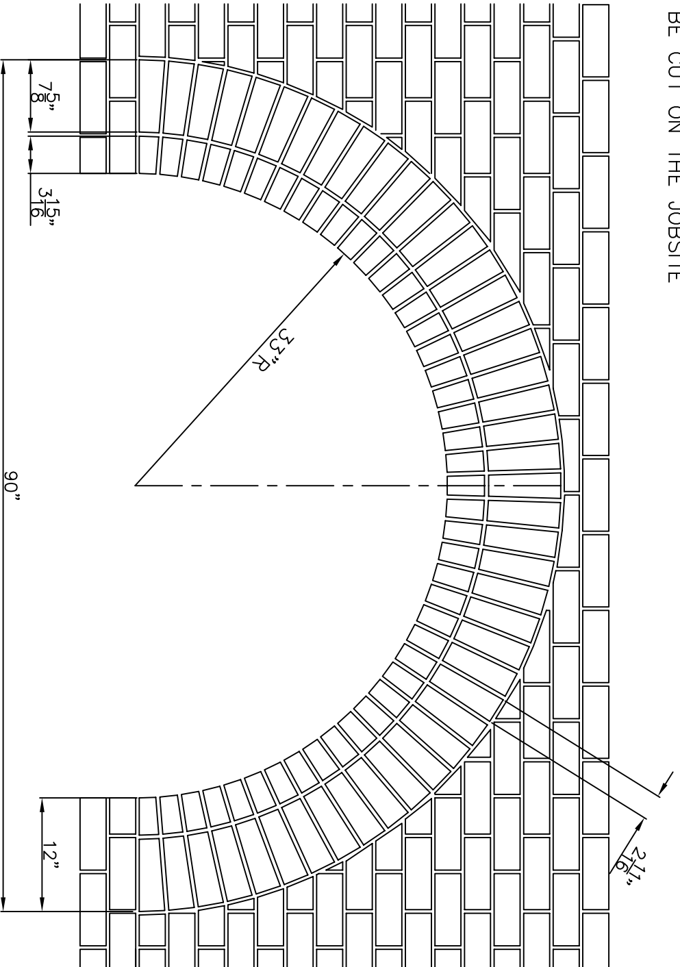
(MASONRY OPENING) SEMICIRCULAR ARCH B BRICK TYPE: MODULAR (12) REQ'D @ 90 PCS. EA.
