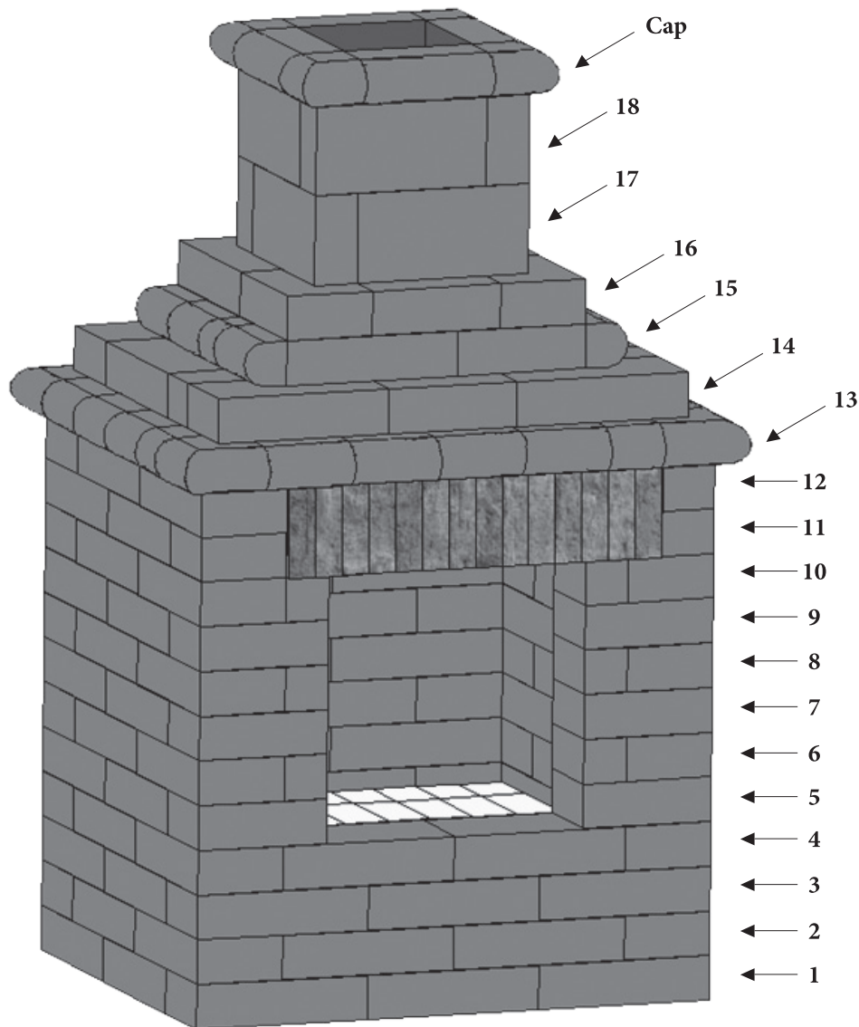
(Fireplace Diagram shown with optional thin brick lintel)
